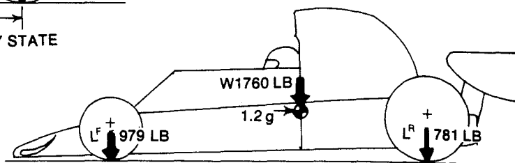
LONGITUDINAL LOAD TRANSFER - BRAKING AT 1.2g RETARDATION
