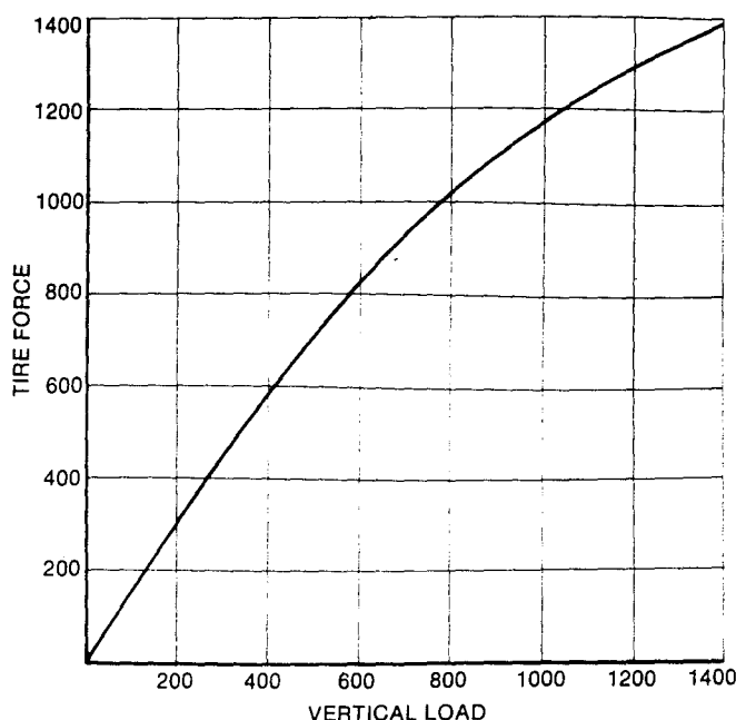
Figure (5): Tire force vs vertical load.
