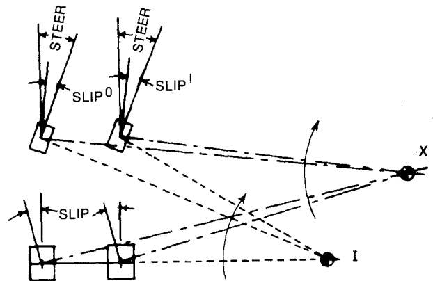
Figure (30): The Ackerman picture modified by slip angle.
