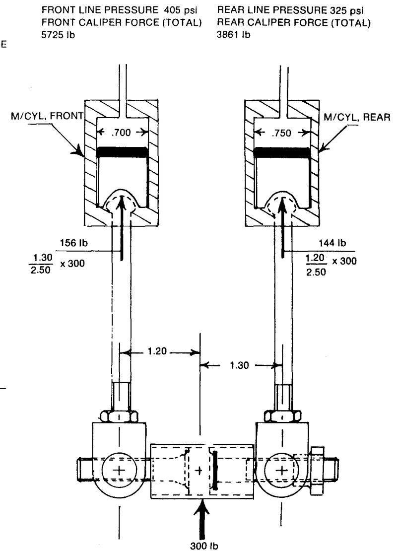
Figure (71b): Bias adjusted 1 turn (.050" with 3/8-24 thread) toward front brakes front to rear force ratio 59.7:40.3.
