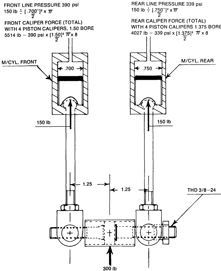
Figure (71a): Bias bar mechanism with bias adjustment in center. Front to rear force ratio 57.8:42.2.
