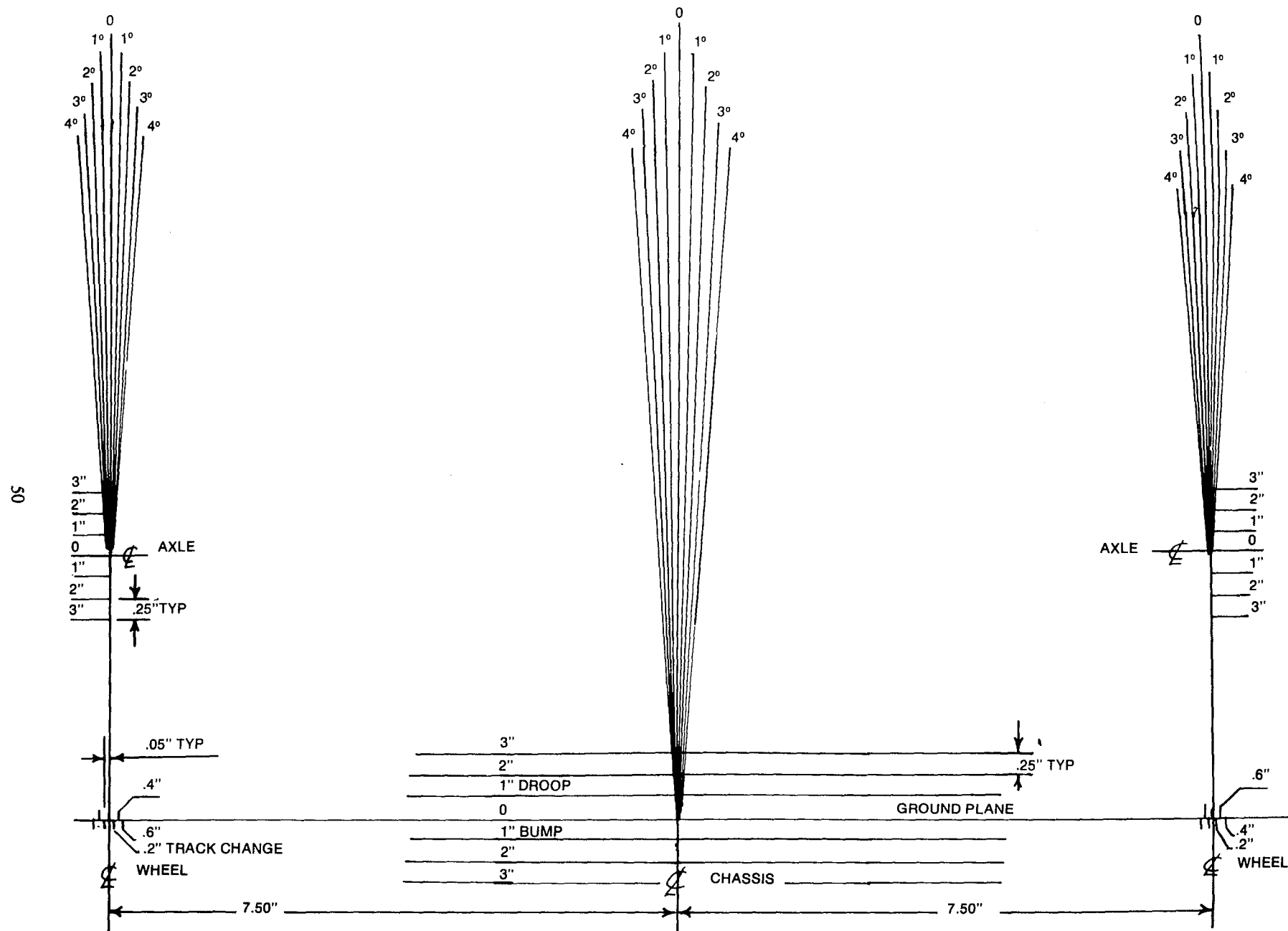
Figure (23a): Background for 1/4 scale suspension geometry model
