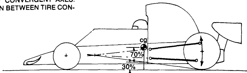
B 30% ANTI-SQUAT BY CONVERGENCE AXES. LINE DRAWN BETWEEN TIRE CONTACT POINT AND CONVERGENCE POINT INTERSECTS PERPENDICULAR FROM cg AT 30% OF cg HEIGHT. SAME PRINCIPLE APPLIES TO ANTI-DIVE.
