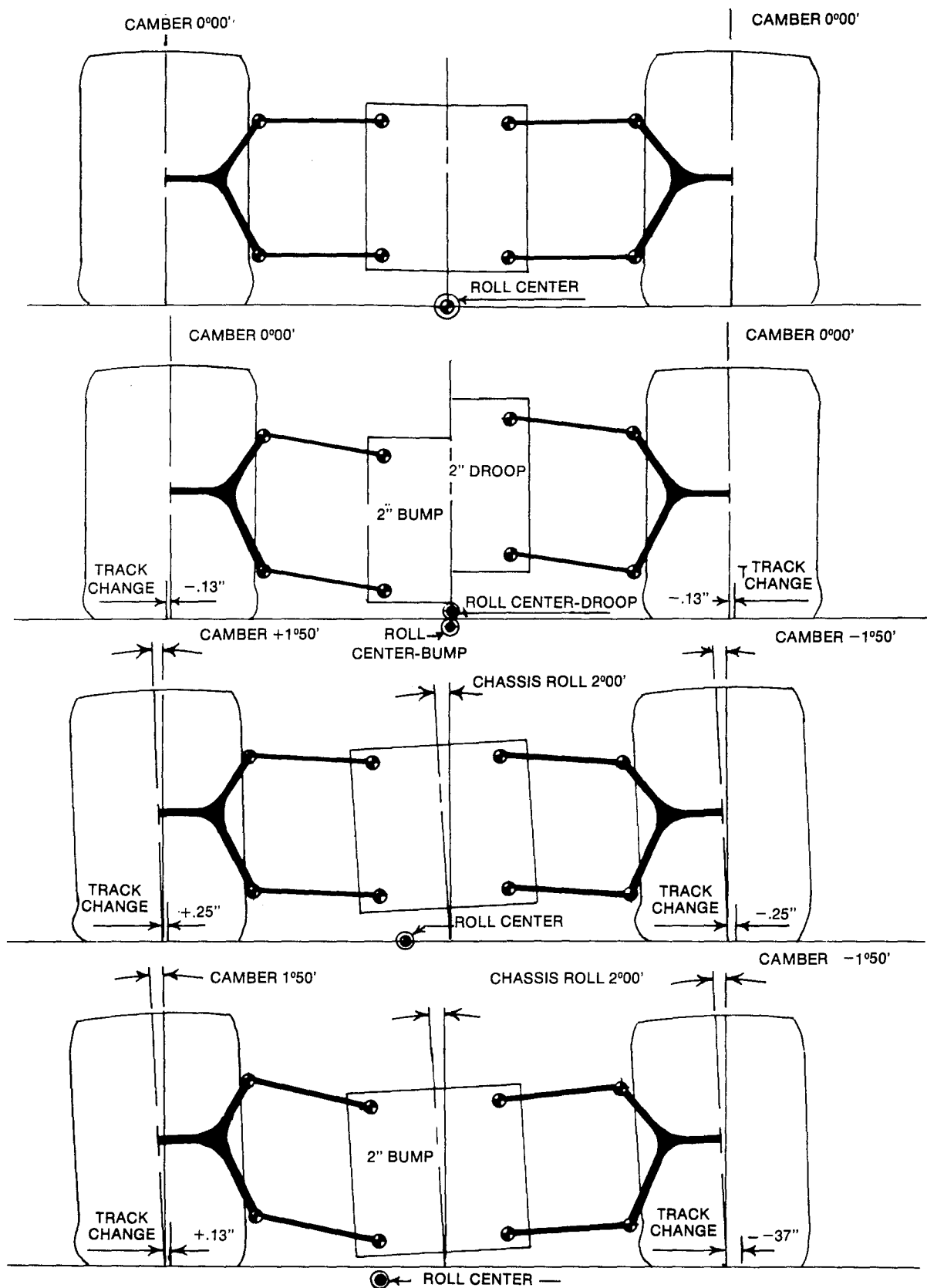
Figure (25): Equal length and parallel link system with relatively long links.
