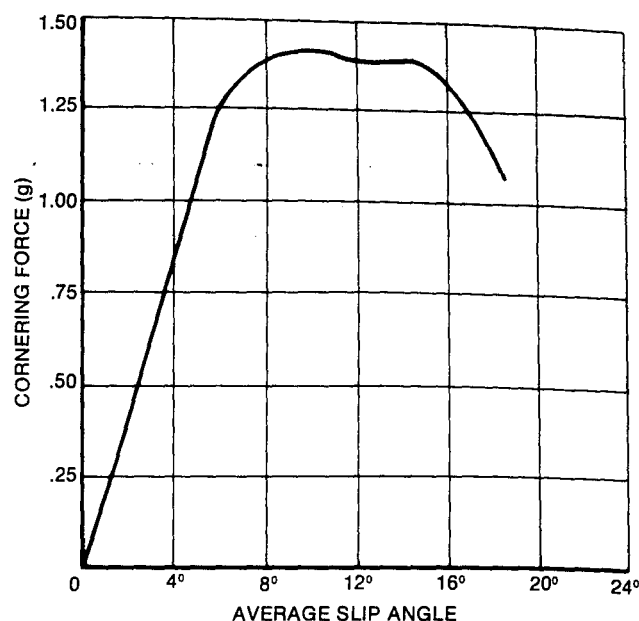
Figure (32): Vehicle cornering force vs average tire slip angle.
