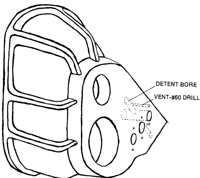
Figure (93): Location of vents for shift rail detents.
