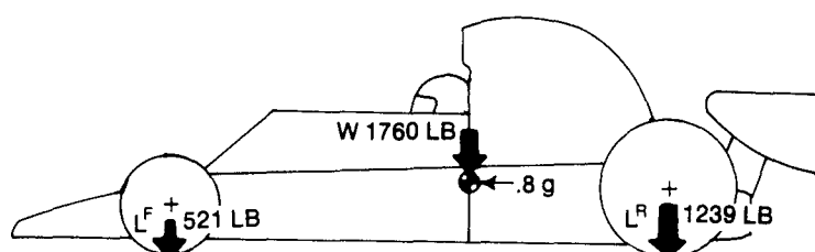
LONGITUDINAL LOAD TRANSFER - ACCELERATION AT 0.8 g
