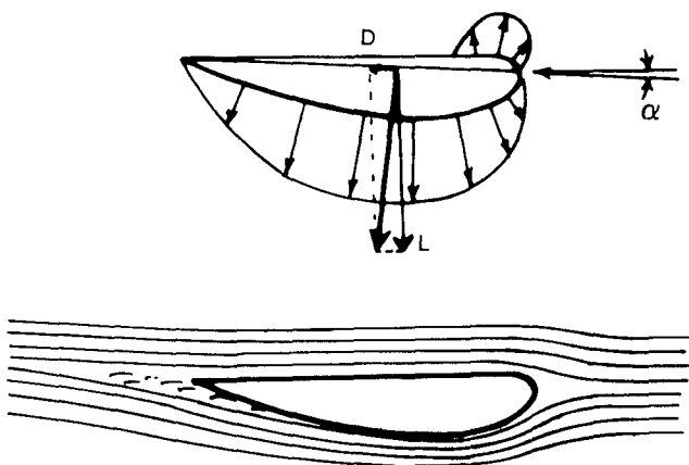
Figure (51a): Pressure vectors, resultant lift and drag vectors and streamlines at low angles of attack.
