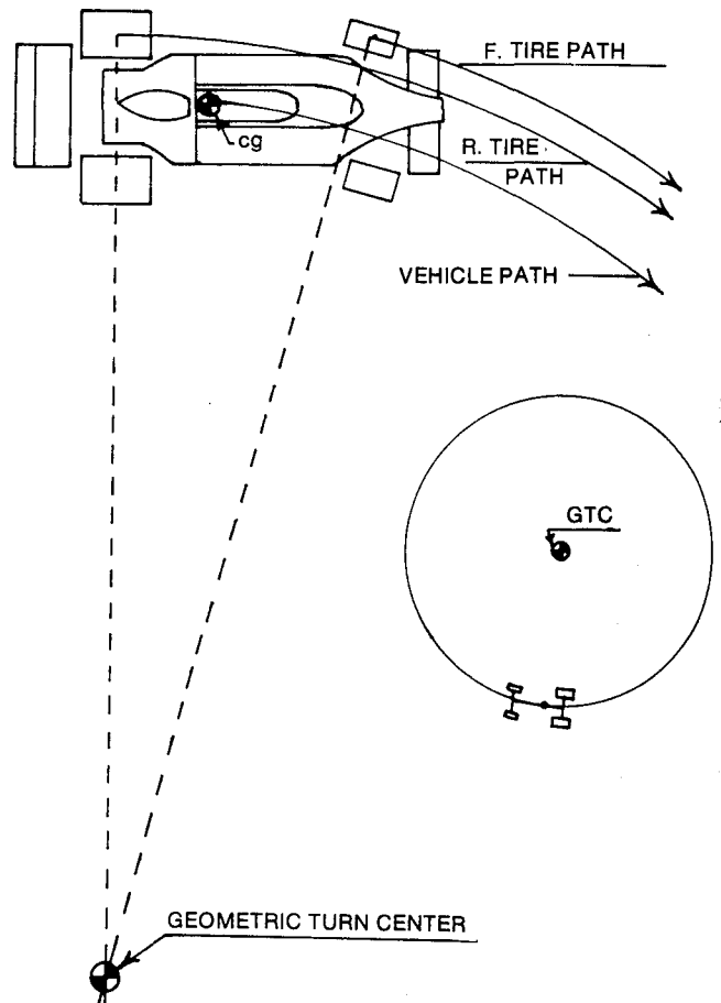
Figure (75): Geometric or Ackerman turn center.
