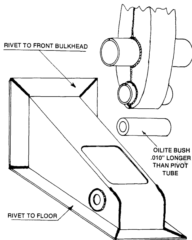
Figure (67a): Boxed brake pedal mount
