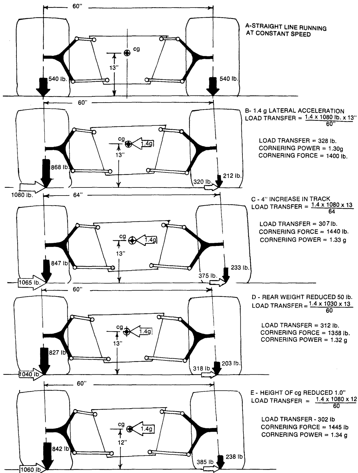
Figure (17): Simplified illustration of the relationship between track width gross weight, center of gravity height and lateral load transfer—and between lateral load transfer and cornering force (Figure 5 used to determine cornering force for given values of vertical load).
