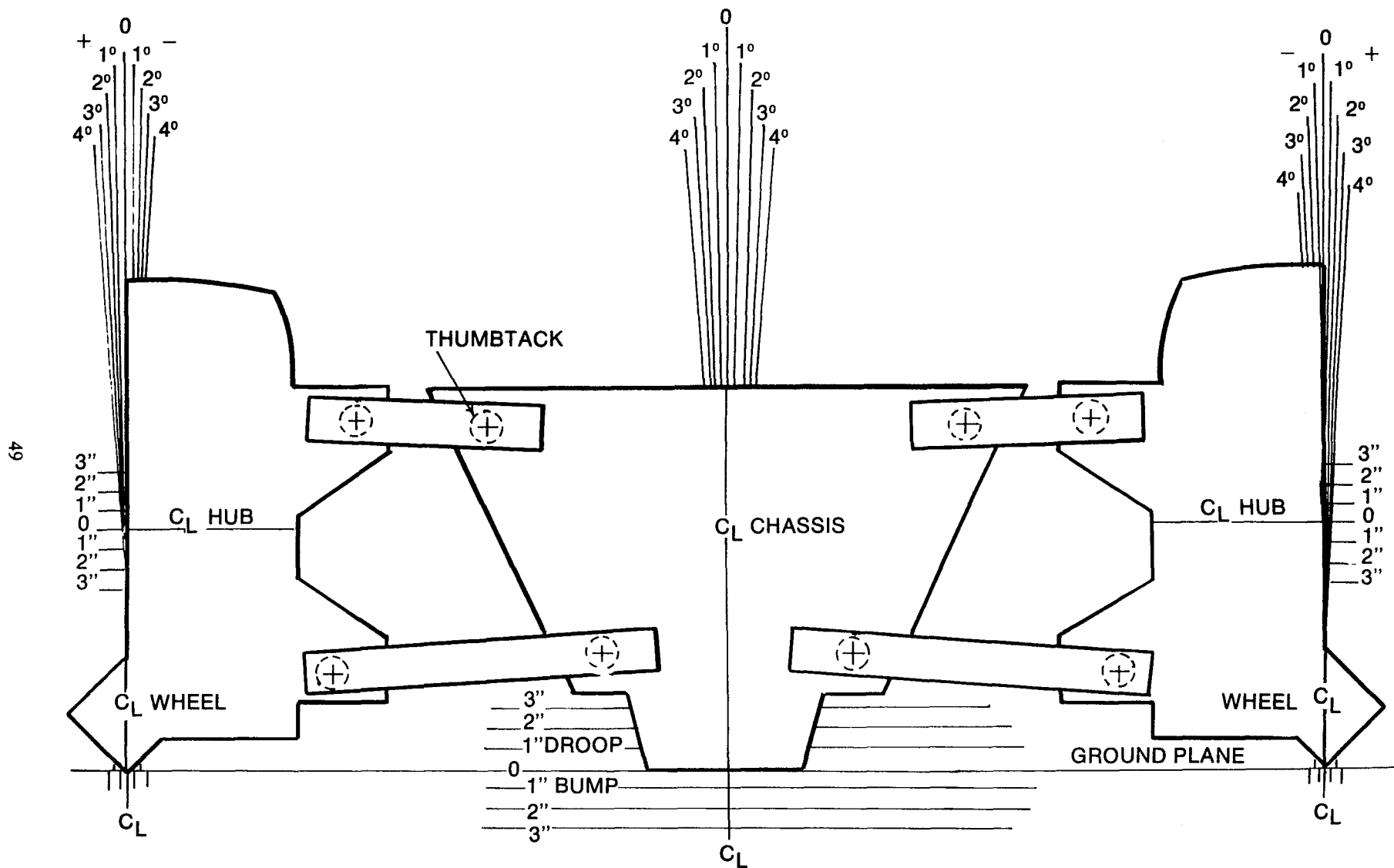
Figure (23): Scale of model of suspension linkage geometry.
