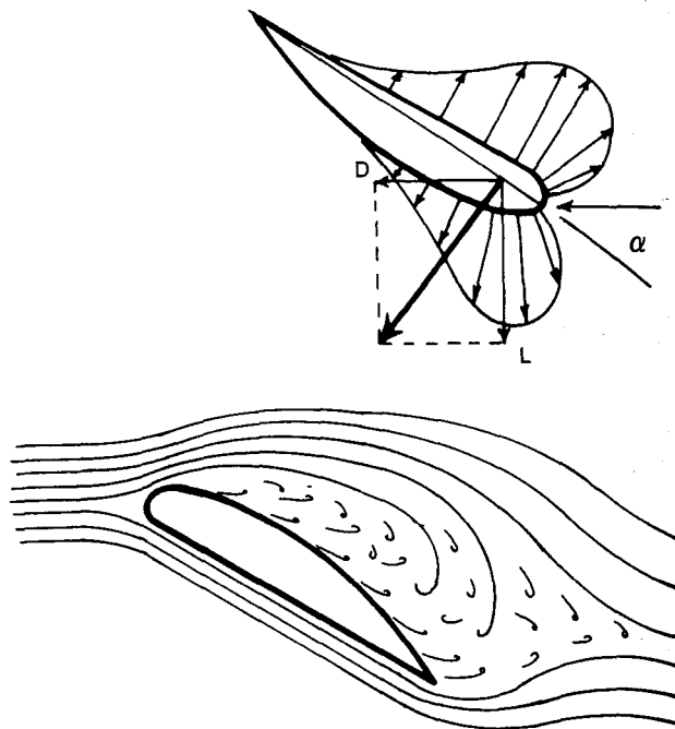
Figure (51c): Pressure vectors, lift/drag and streamlines at high angle of attack—wing stalled.
