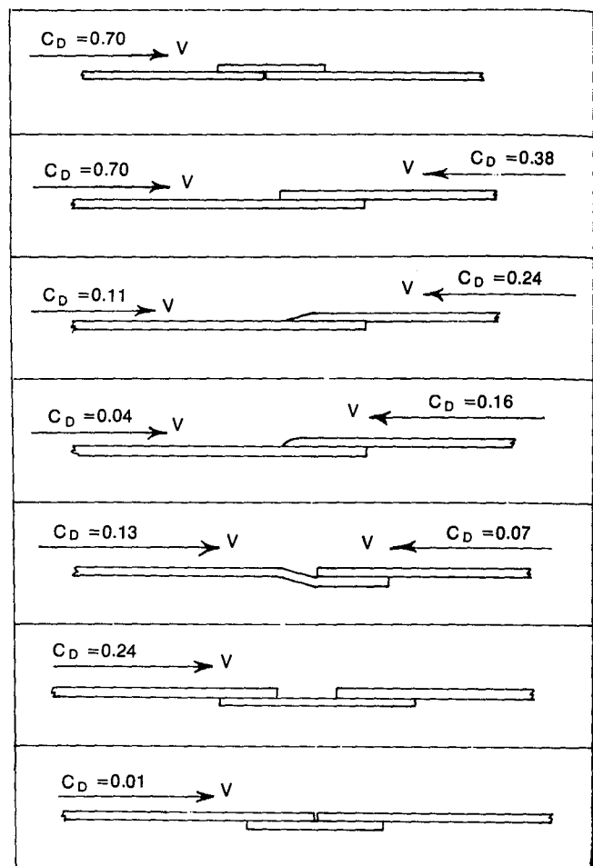
Figure (47): Independent drag coefficient of various sheet metal joints. Sheet thickness is constant.
