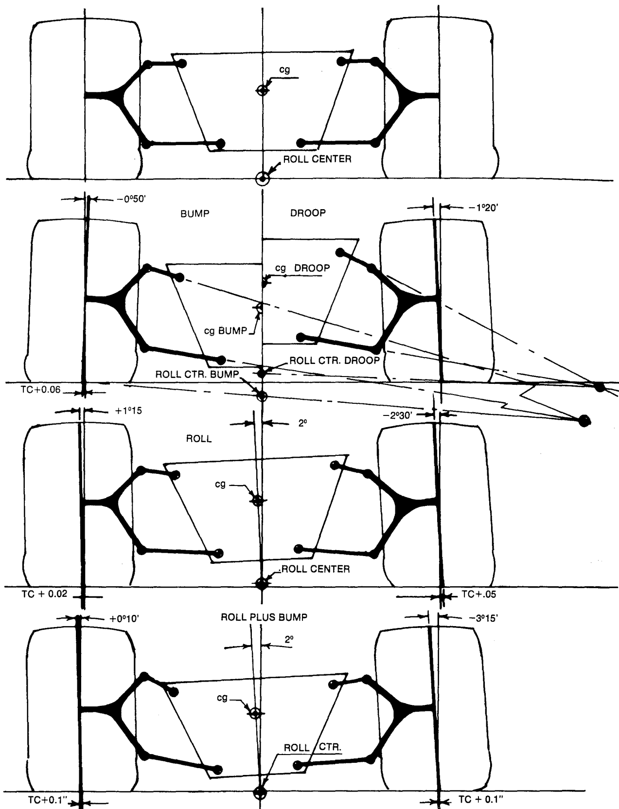
Figure (26): Unequal length parallel links.
