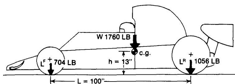
LONGITUDINAL LOAD DISTRIBUTION - STEADY STATE
