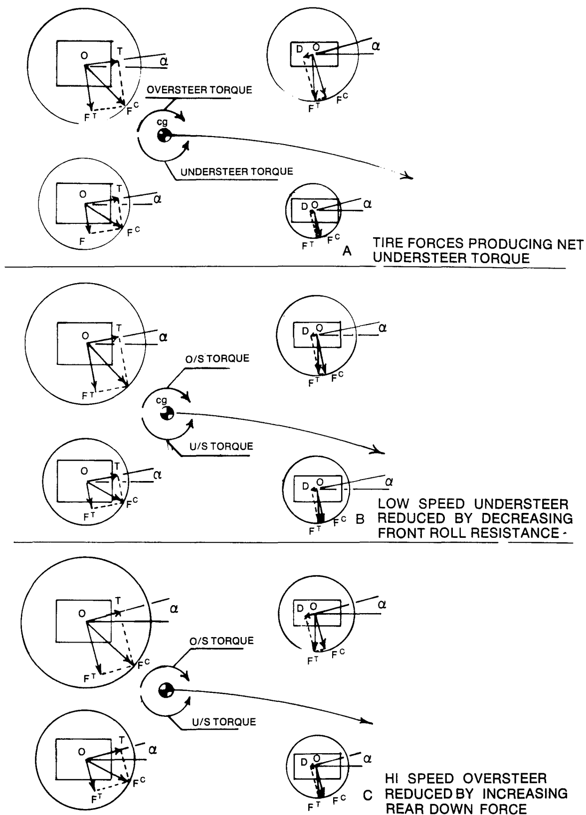
Figure (84): Tire forces producing understeer and oversteer torques about vehicle's center of gravity.
