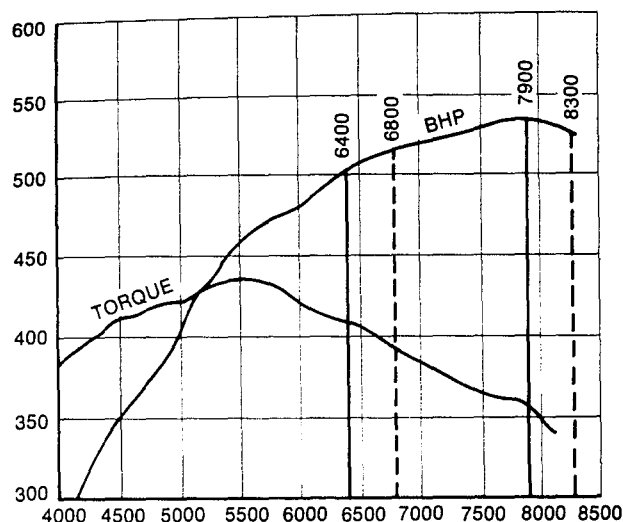
Figure (89a): Typical 5 litre BHP and torque curves.
