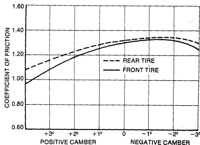
Figure (6): Camber angle vs coefficient of friction.
