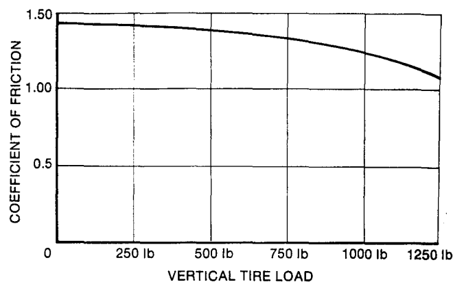
Figure (4): Coefficient of friction vs vertical tire load.
