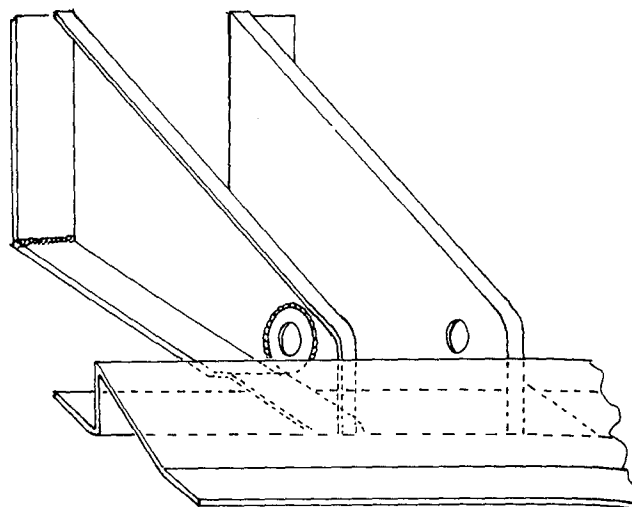
Figure (67b): Flanged brake pedal mount.
