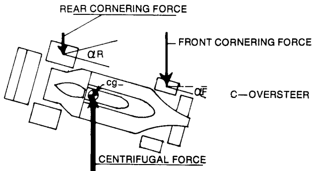
Figure (74): Balance of forces between front and rear tire cornering forces resulting in neutral steer, understeer and oversteer.
