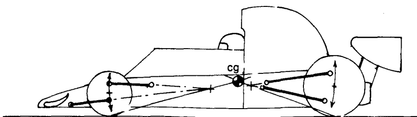
A 100% ANTI-DIVE & 100% ANTI-SQUAT BY CONVERGENT AXES. CONVERGENCE POINTS LIE ON LINES DRAWN BETWEEN TIRE CONTACT POINT & SPRUNG MASS CENTER OF GRAVITY
