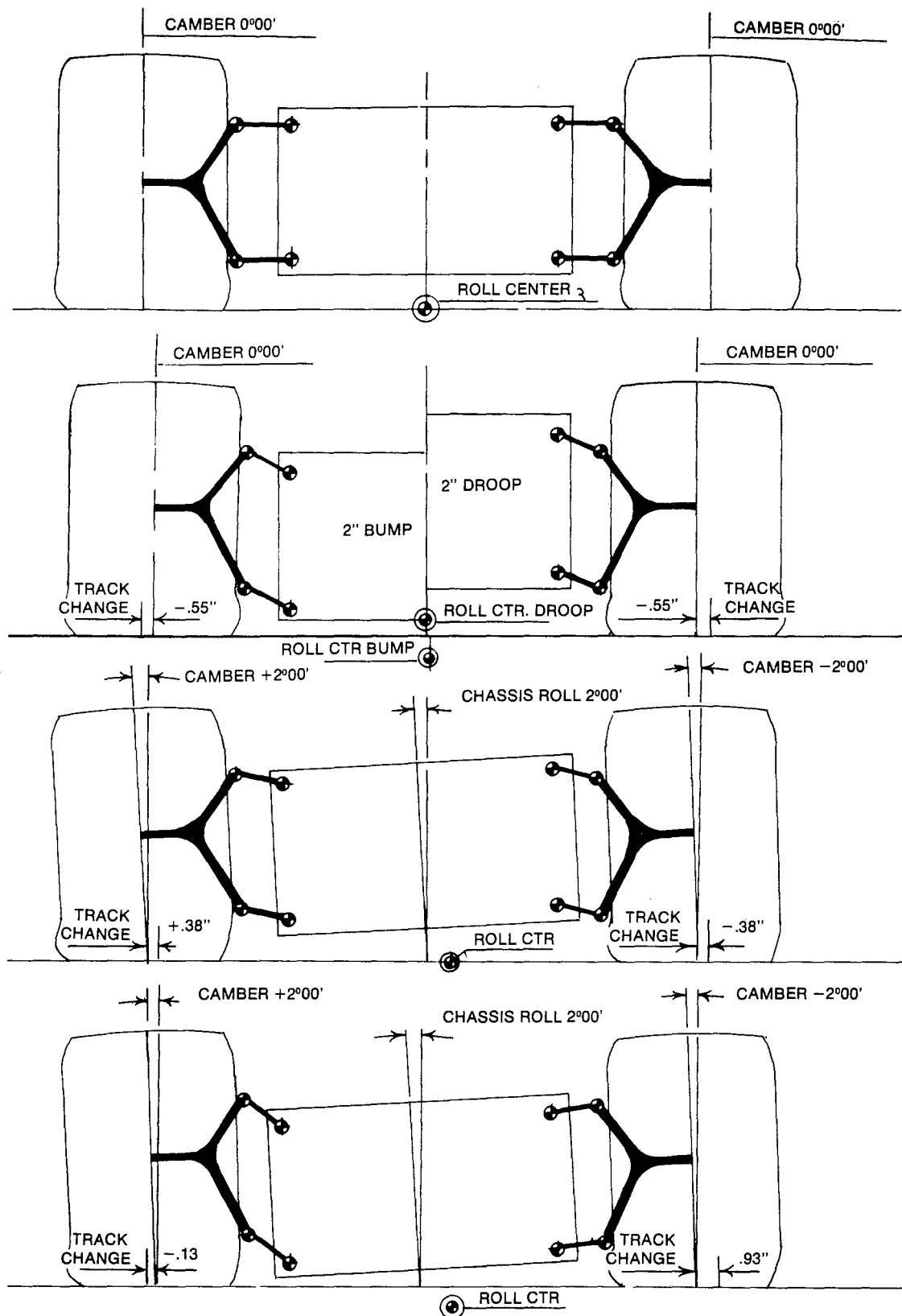
Figure (24): Equal length and parallel link system with short links.
