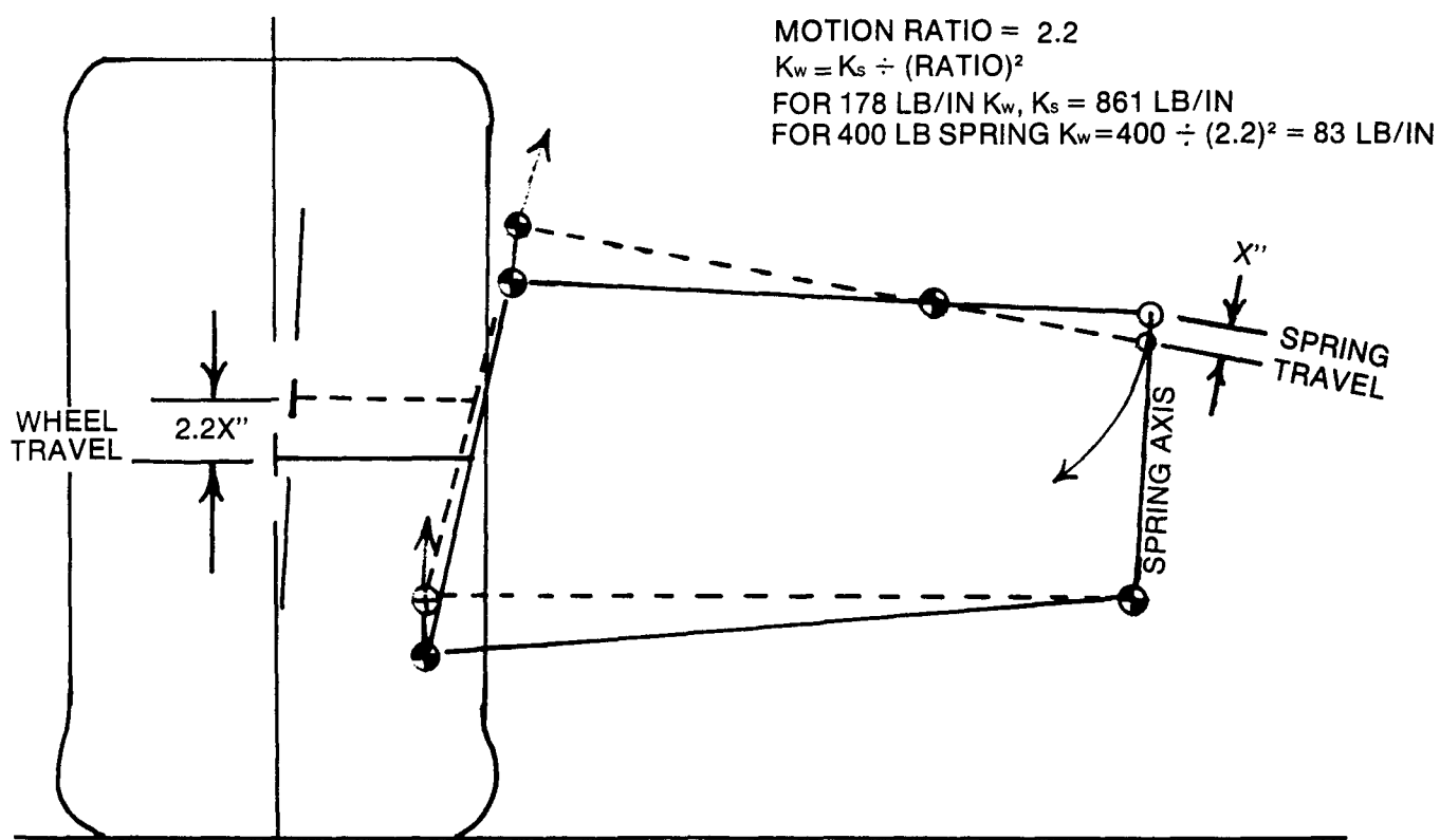
Figure (35): Wheel rate vs spring rate—inboard suspension.
